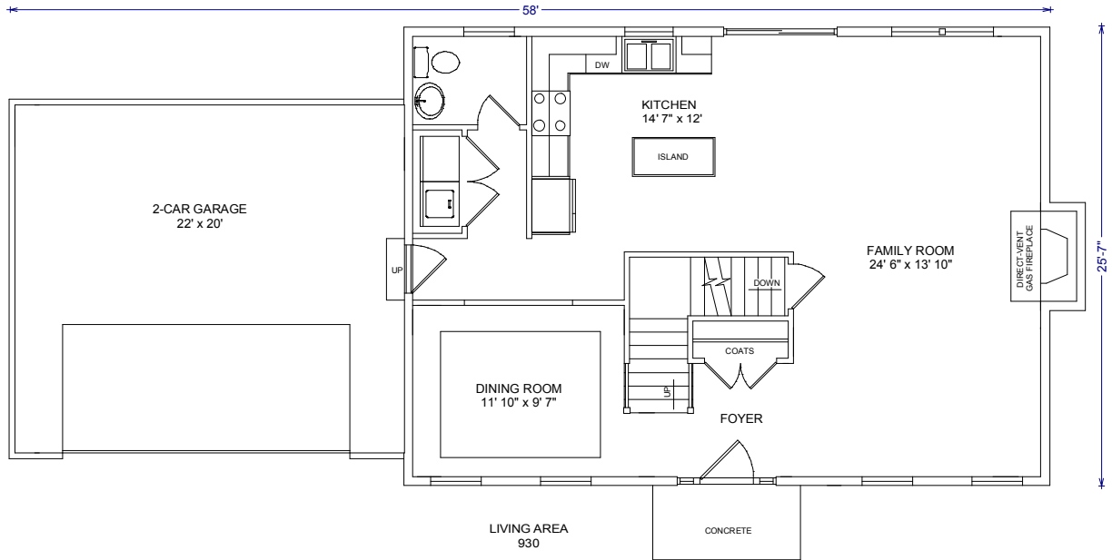
First Floor
