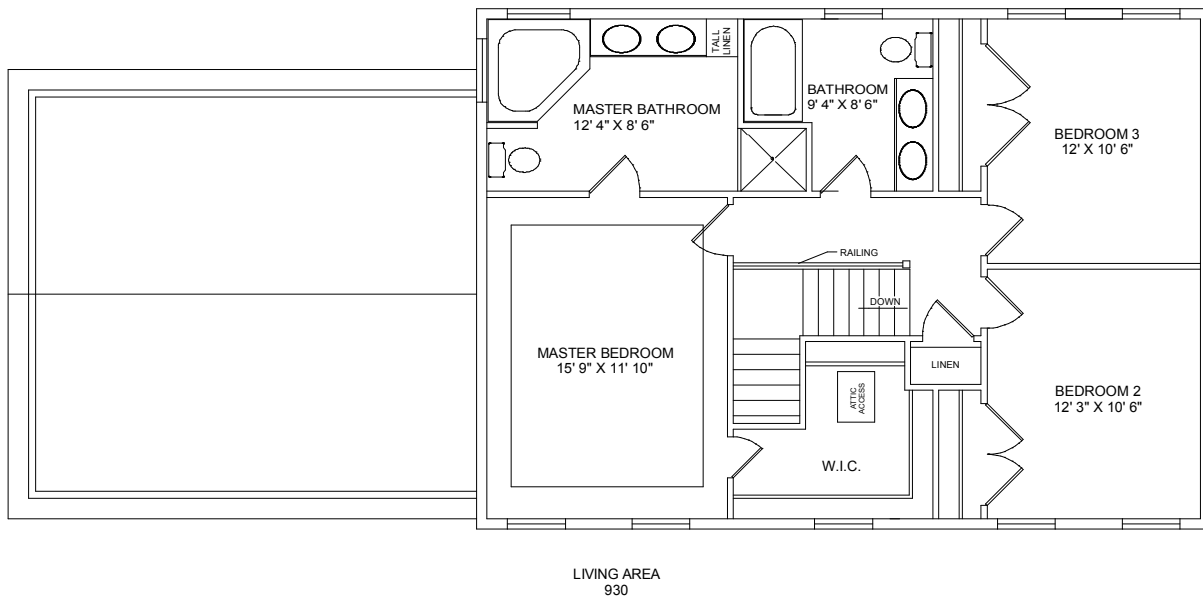
Second Floor
